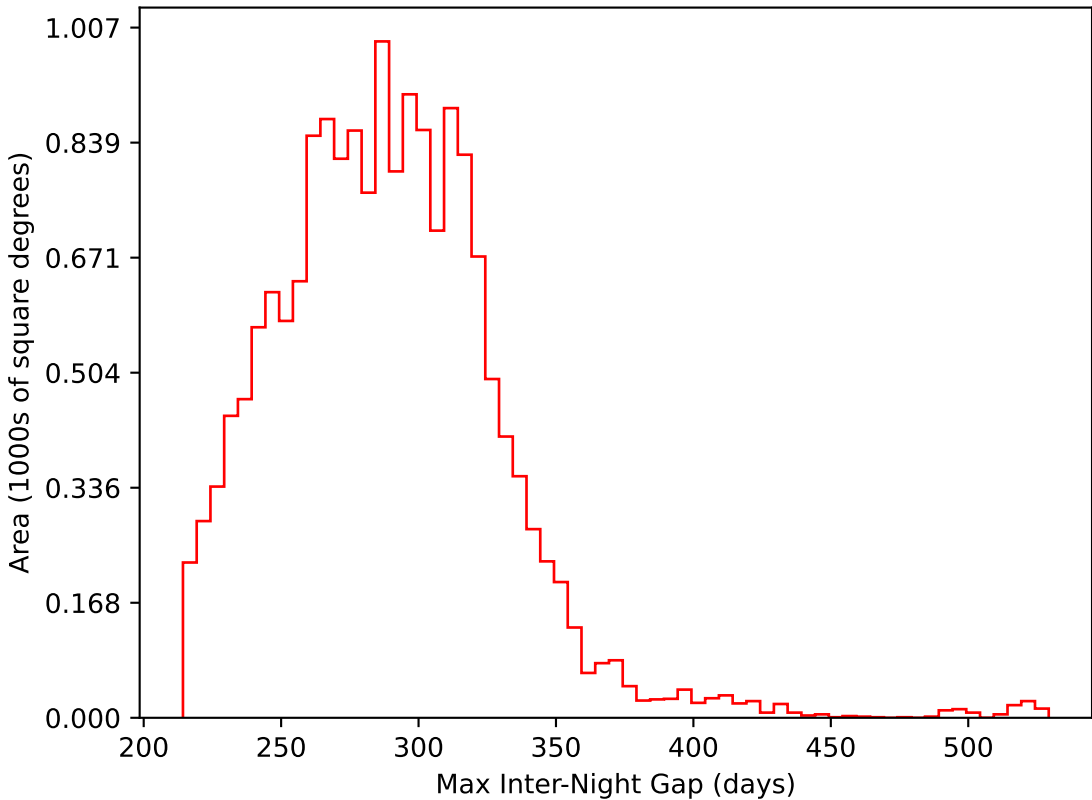
too_elab_r32_d3_giz_v3.4_10yrs WFD i band: Max Inter-Night Gap
