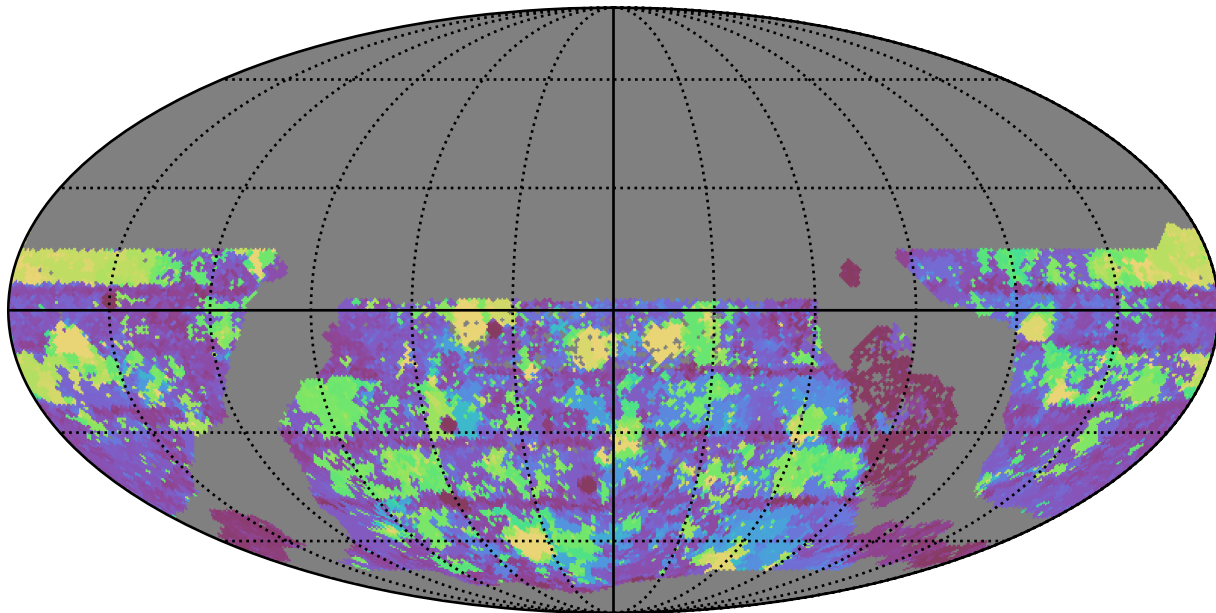
too_elab_r32_d3_giz_v3.4_10yrs WFD g band: Max Inter-Night Gap
