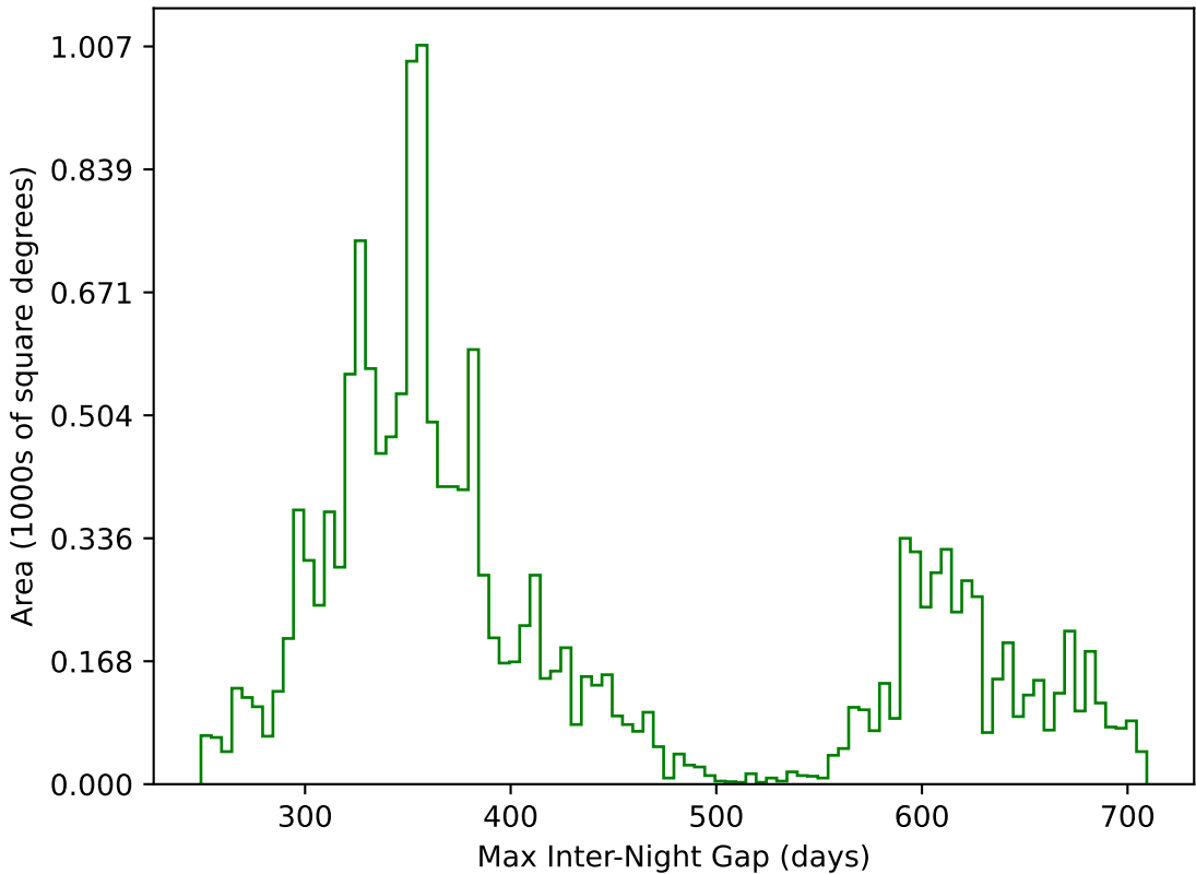
too_elab_r32_d3_giz_v3.4_10yrs WFD g band: Max Inter-Night Gap
