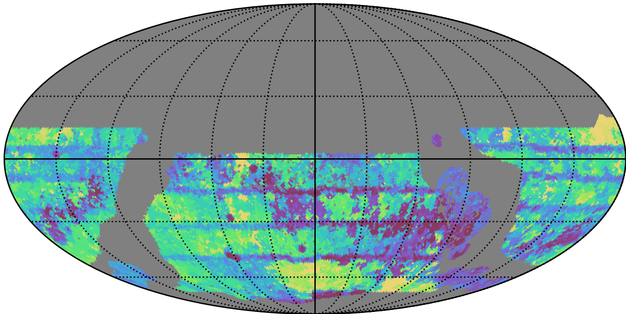
too_elab_r32_d3_giz_v3.4_10yrs WFD all bands: Max Inter-Night Gap
