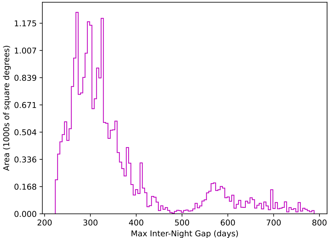
too_elab_r32_d3_giz_v3.4_10yrs All sky z band: Max Inter-Night Gap
