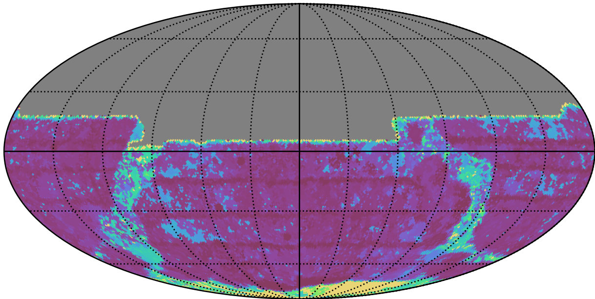
too_elab_r32_d3_giz_v3.4_10yrs All sky y band: Max Inter-Night Gap
