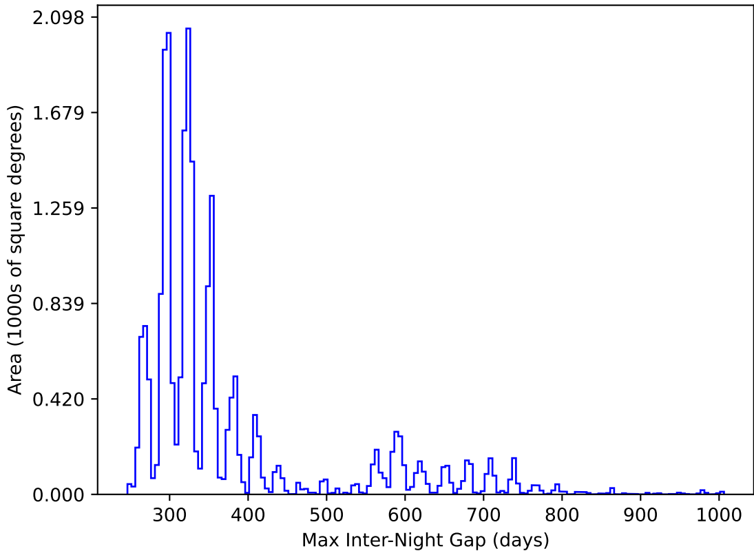
too_elab_r32_d3_giz_v3.4_10yrs All sky y band: Max Inter-Night Gap
