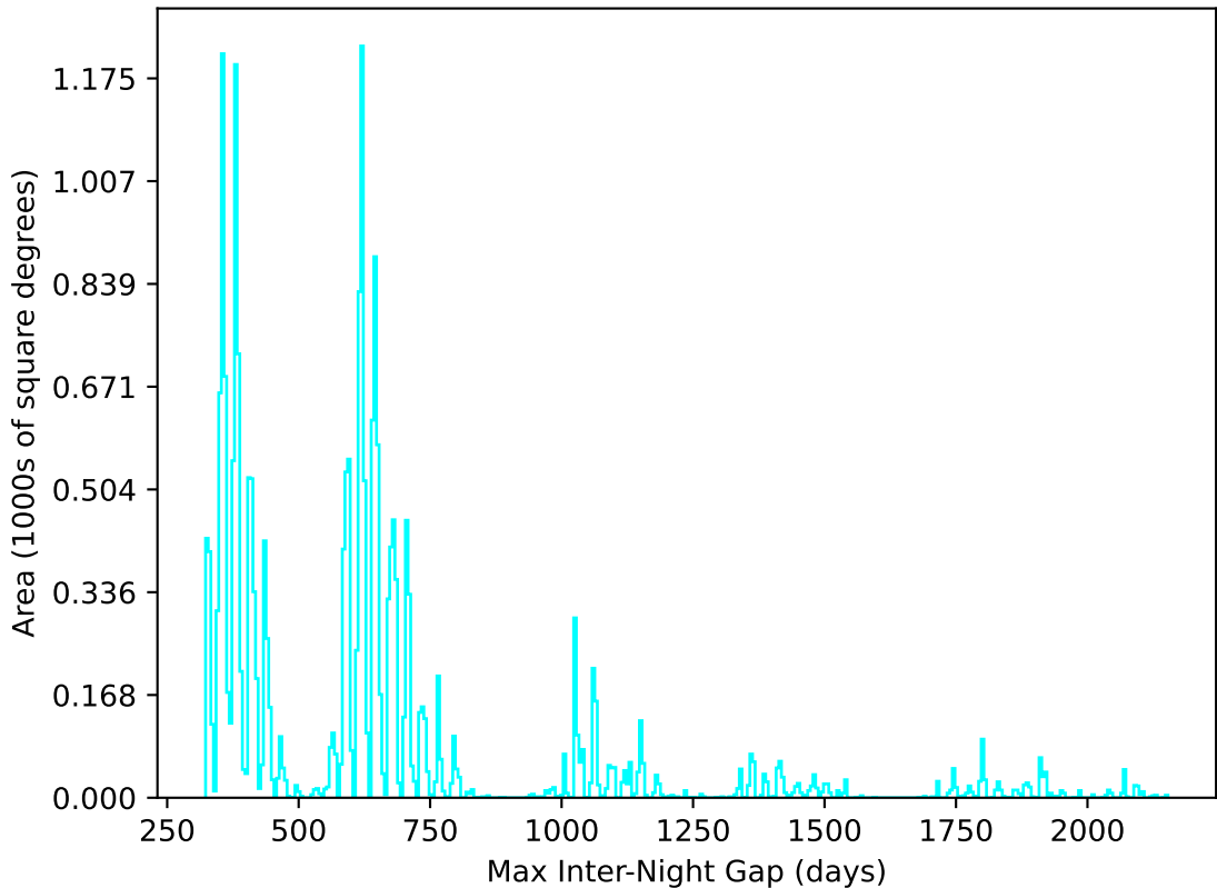
too_elab_r32_d3_giz_v3.4_10yrs All sky u band: Max Inter-Night Gap
