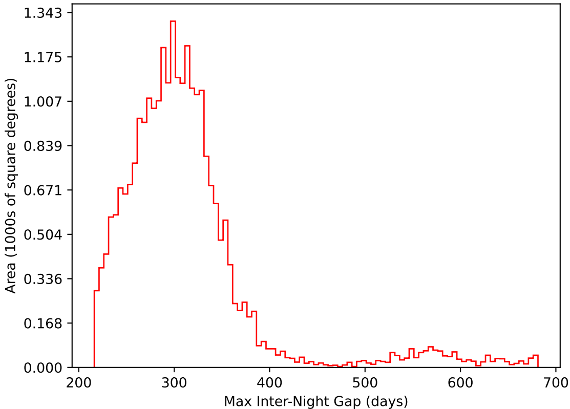
too_elab_r32_d3_giz_v3.4_10yrs All sky i band: Max Inter-Night Gap
