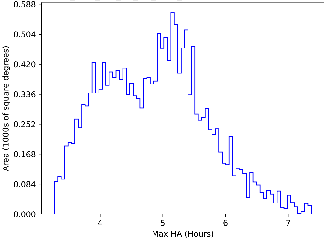
too_elab_r32_d3_giz_v3.4_10yrs WFD z band: Max HA
