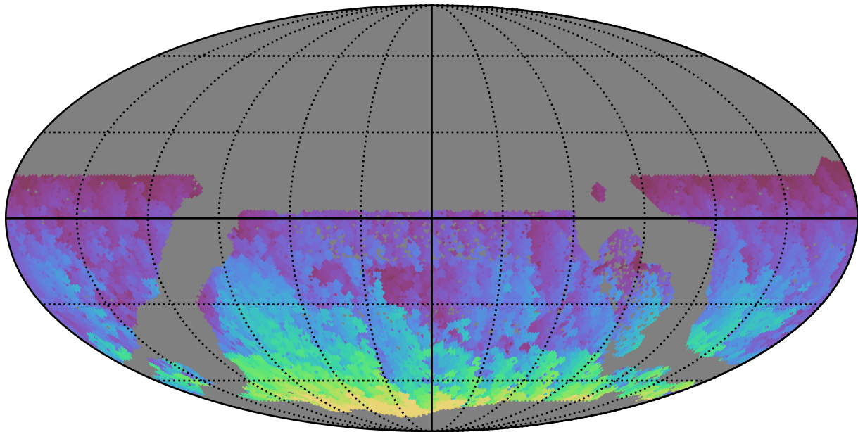
too_elab_r32_d3_giz_v3.4_10yrs WFD y band: Max HA
