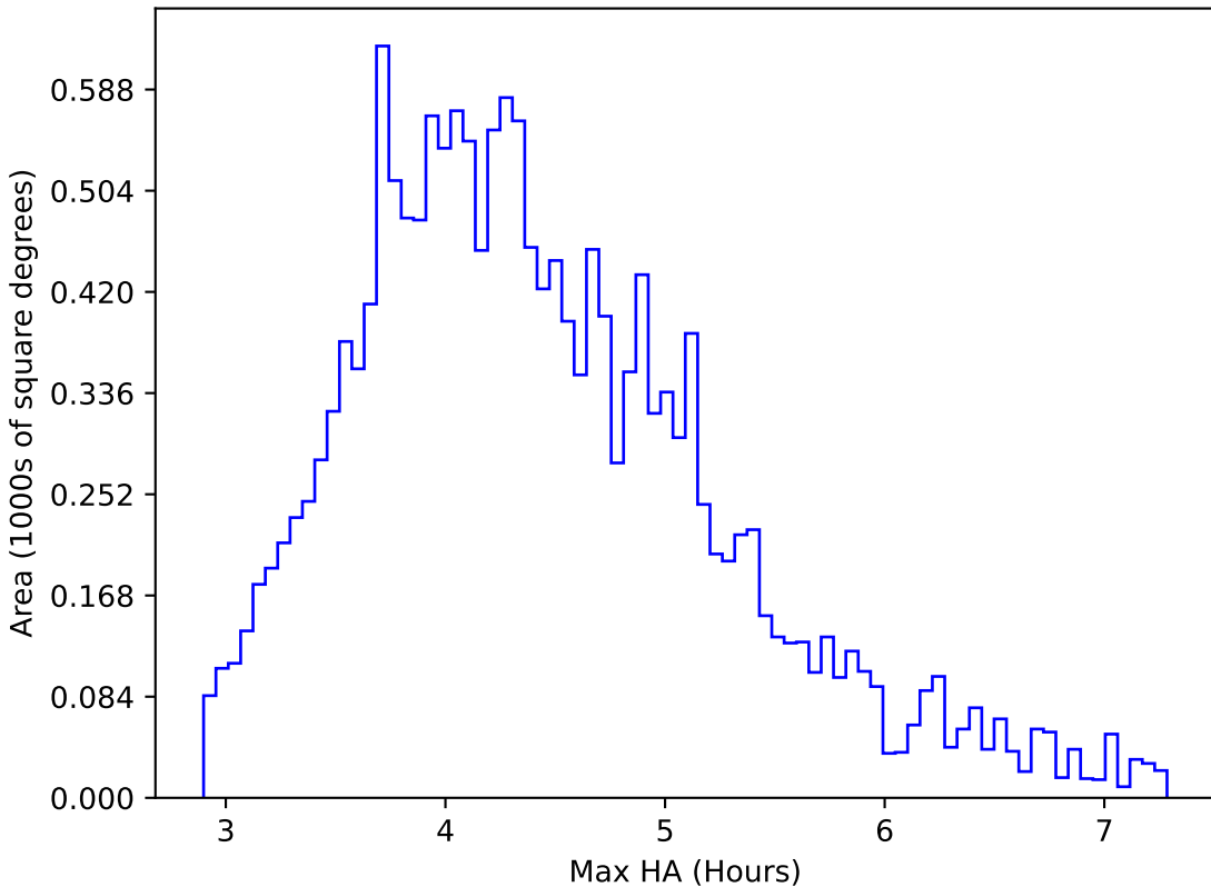
too_elab_r32_d3_giz_v3.4_10yrs WFD r band: Max HA
