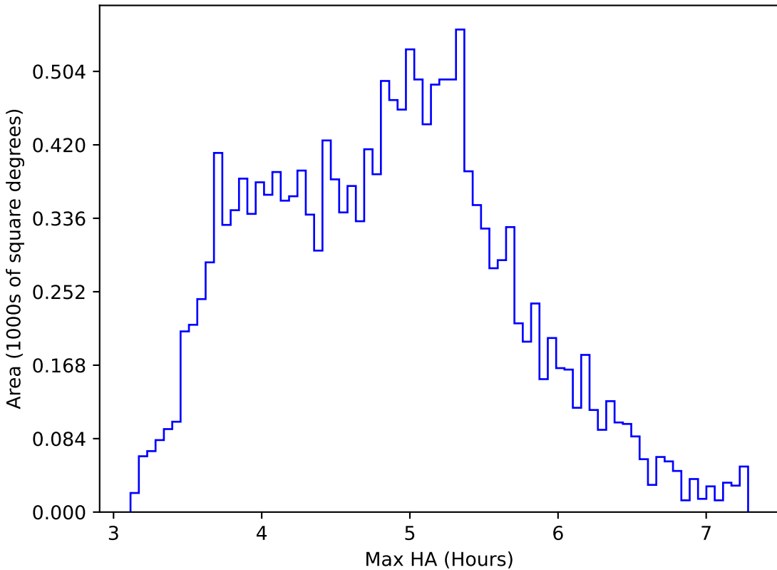
too_elab_r32_d3_giz_v3.4_10yrs WFD i band: Max HA
