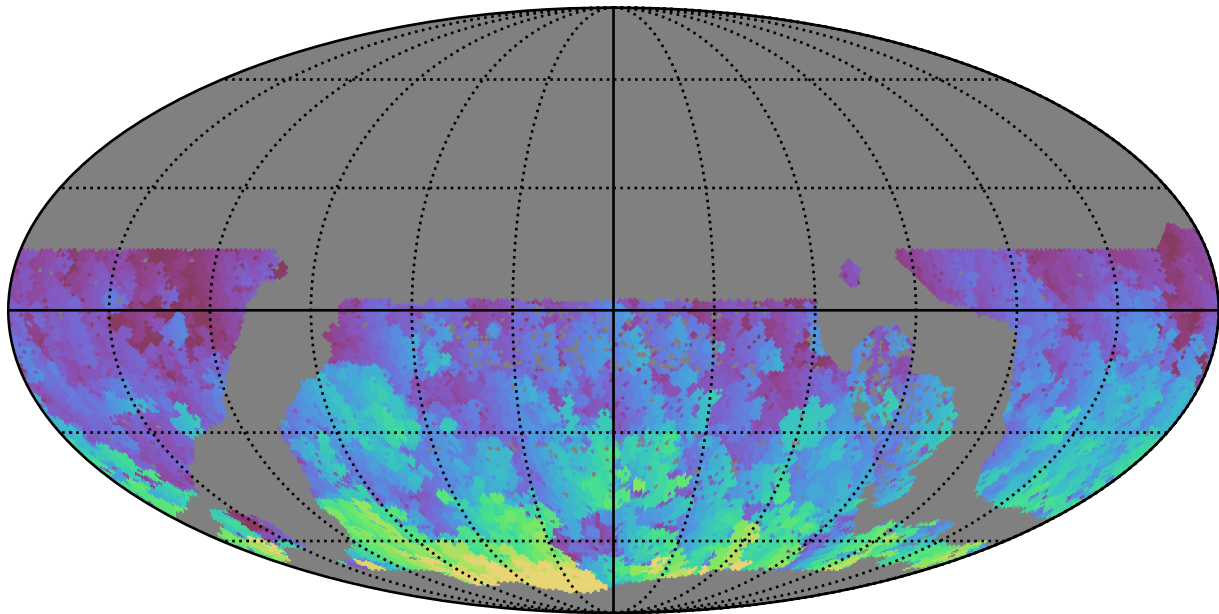
too_elab_r32_d3_giz_v3.4_10yrs WFD g band: Max HA
