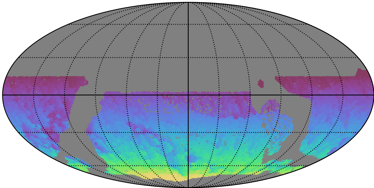
too_elab_r32_d3_giz_v3.4_10yrs WFD all bands: Max HA
