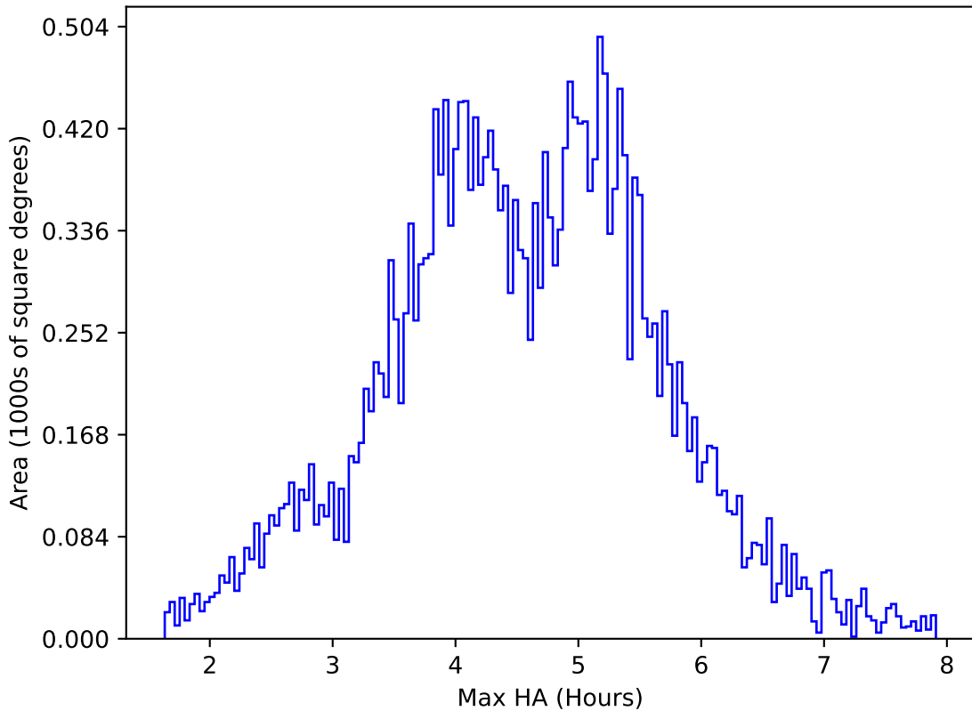
too_elab_r32_d3_giz_v3.4_10yrs All sky z band: Max HA
