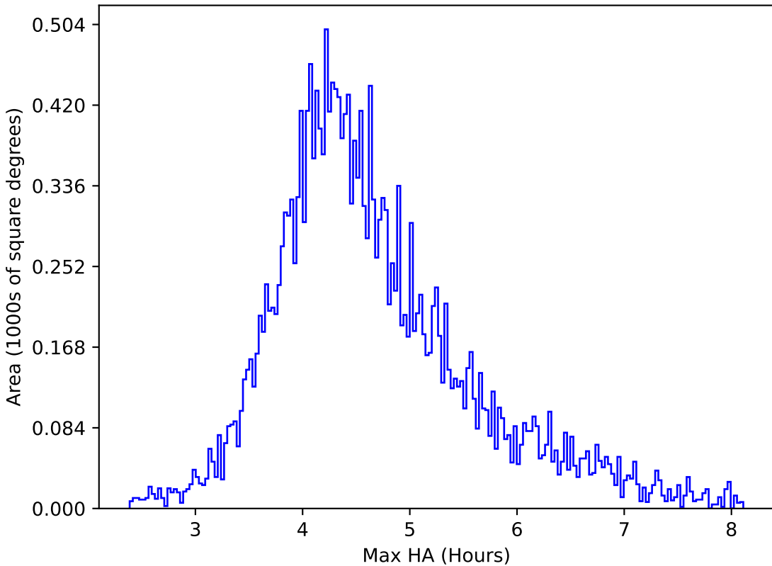
too_elab_r32_d3_giz_v3.4_10yrs All sky y band: Max HA
