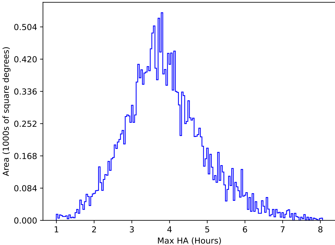
too_elab_r32_d3_giz_v3.4_10yrs All sky u band: Max HA
