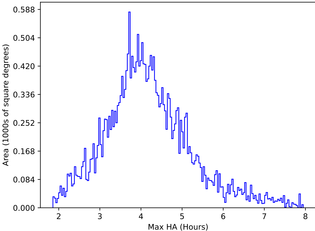
too_elab_r32_d3_giz_v3.4_10yrs All sky r band: Max HA
