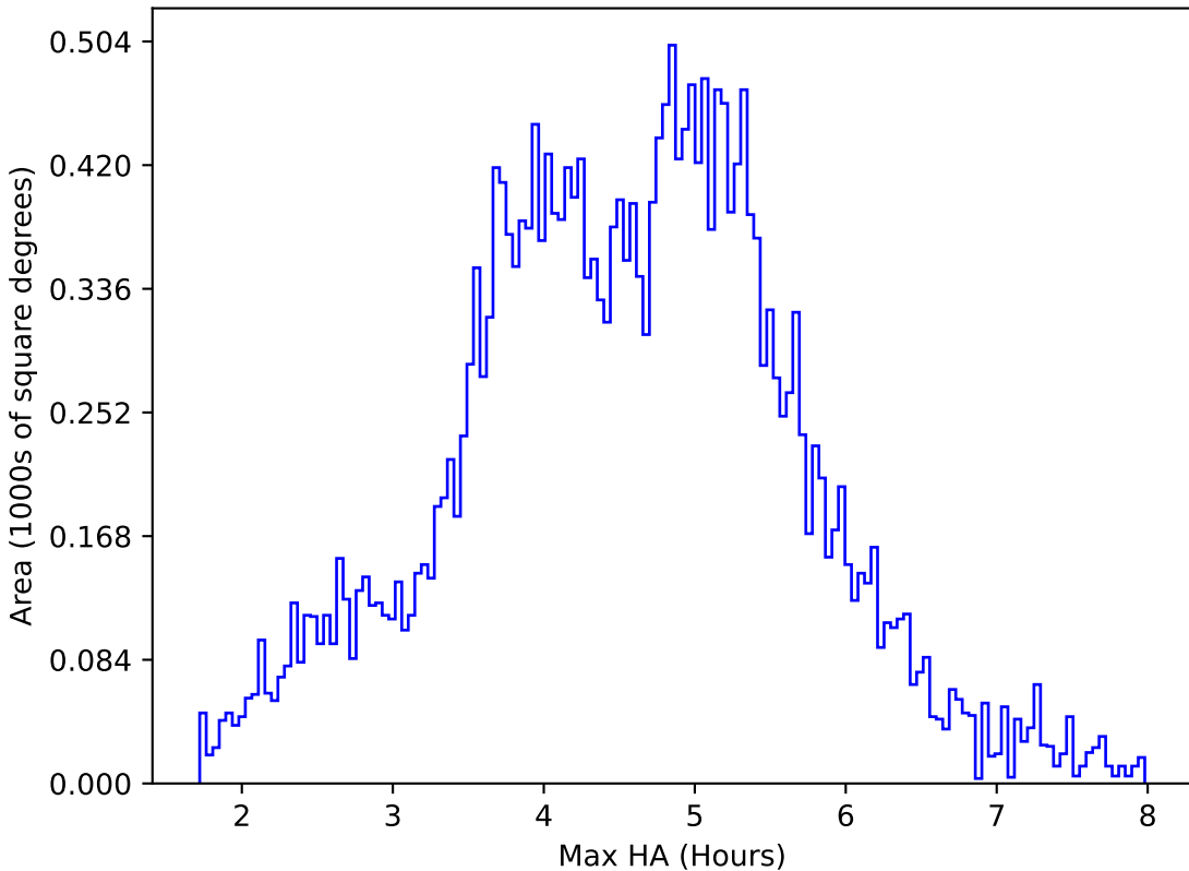
too_elab_r32_d3_giz_v3.4_10yrs All sky i band: Max HA
