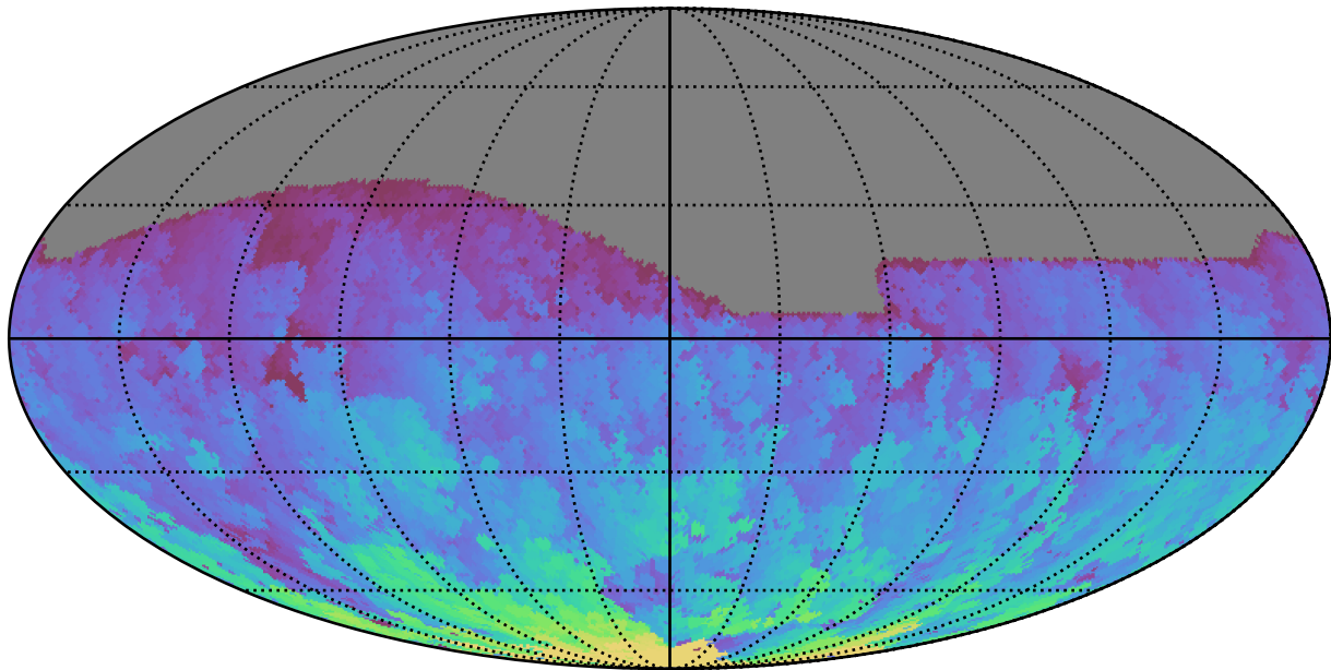
too_elab_r32_d3_giz_v3.4_10yrs All sky g band: Max HA
