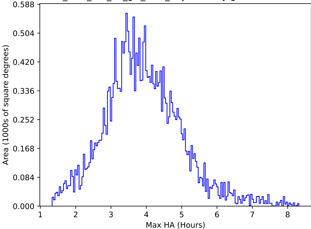
too_elab_r32_d3_giz_v3.4_10yrs All sky g band: Max HA
