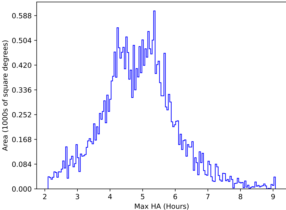
too_elab_r32_d3_giz_v3.4_10yrs All sky all bands: Max HA
