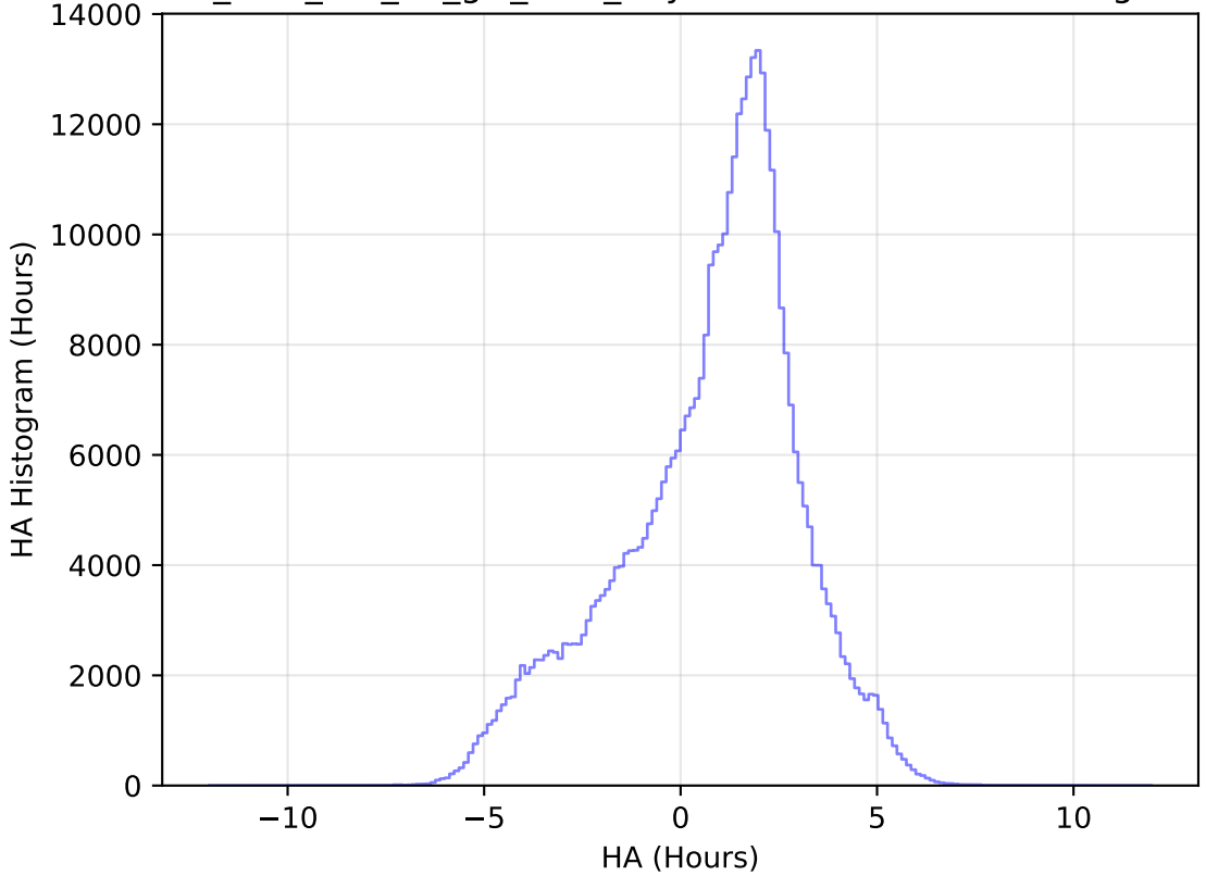
too_elab_r32_d3_giz_v3.4_10yrs WFD z band: HA Histogram
