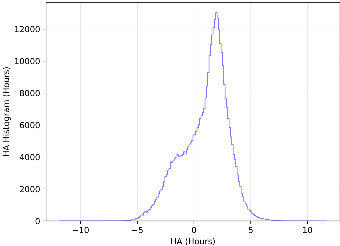
too_elab_r32_d3_giz_v3.4_10yrs WFD y band: HA Histogram
