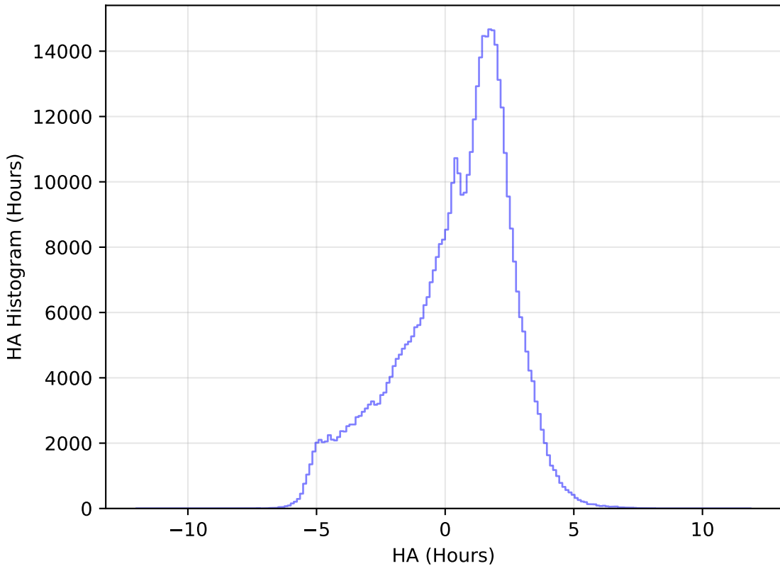
too_elab_r32_d3_giz_v3.4_10yrs WFD r band: HA Histogram
