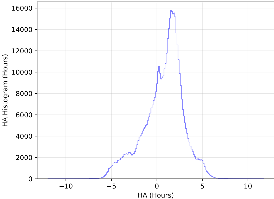
too_elab_r32_d3_giz_v3.4_10yrs WFD i band: HA Histogram
