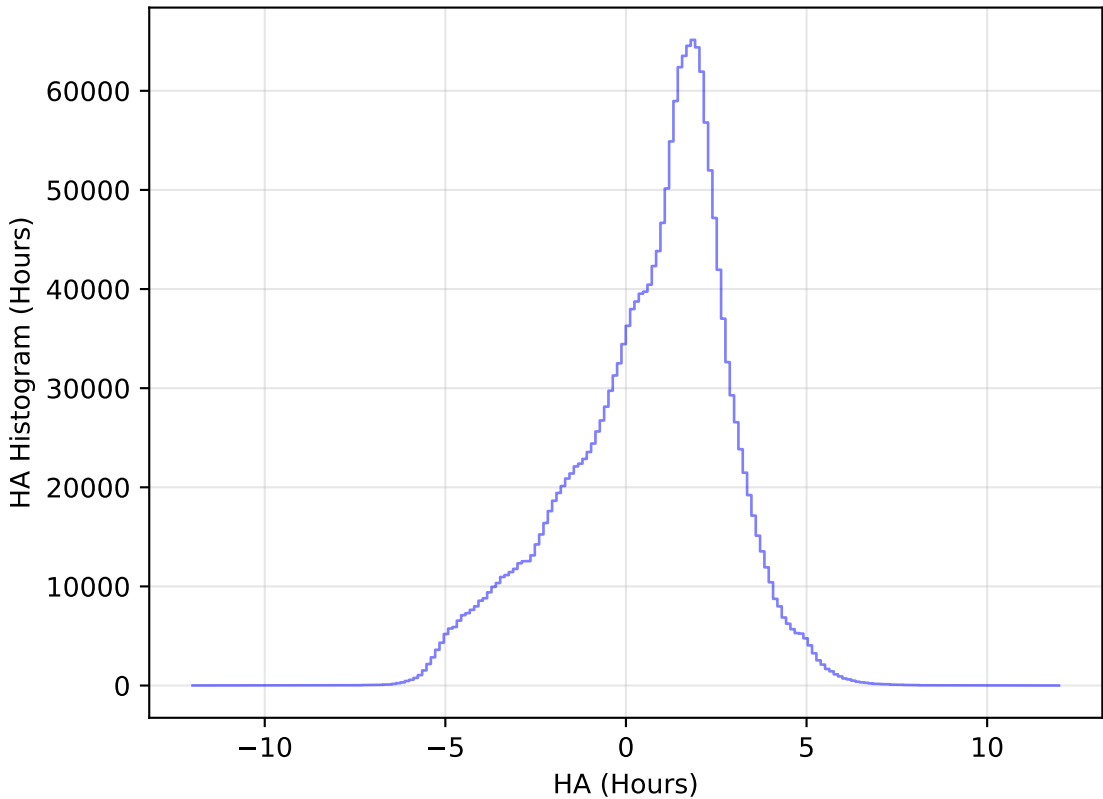
too_elab_r32_d3_giz_v3.4_10yrs WFD all bands: HA Histogram
