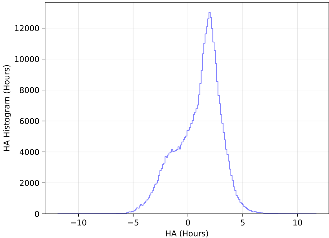
too_elab_r32_d3_giz_v3.4_10yrs All sky y band: HA Histogram
