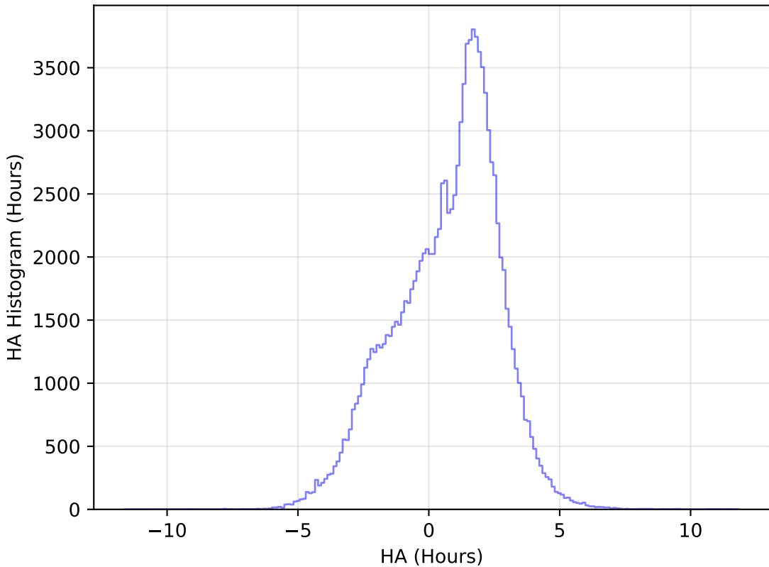
too_elab_r32_d3_giz_v3.4_10yrs All sky u band: HA Histogram
