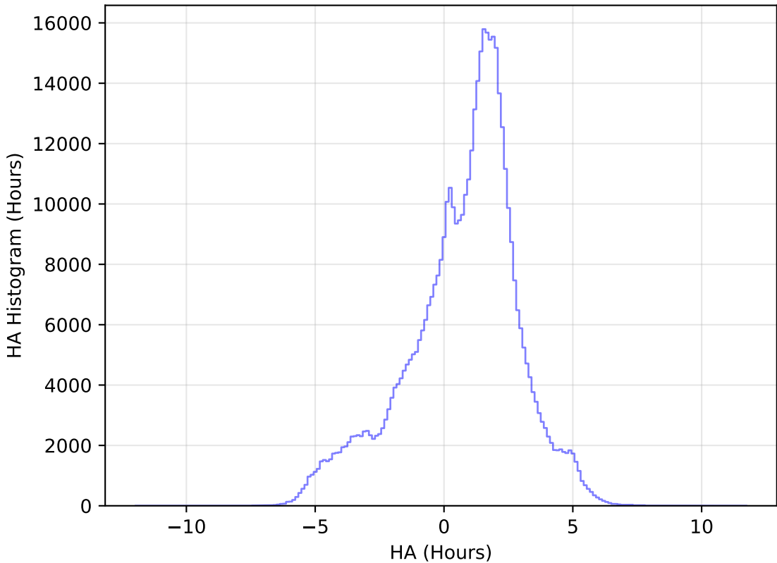
too_elab_r32_d3_giz_v3.4_10yrs All sky i band: HA Histogram
