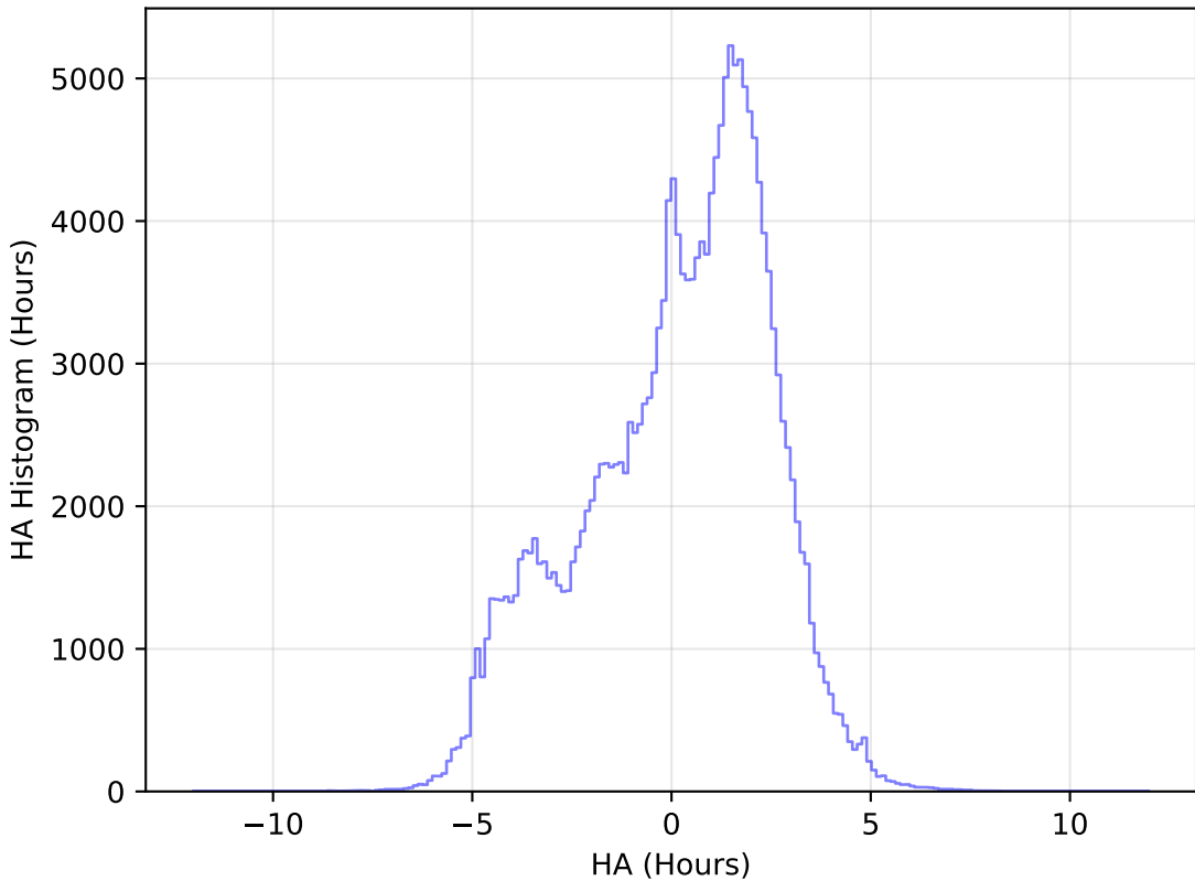
too_elab_r32_d3_giz_v3.4_10yrs All sky g band: HA Histogram
