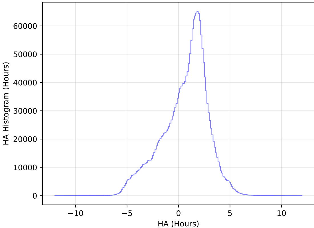
too_elab_r32_d3_giz_v3.4_10yrs All sky all bands: HA Histogram
