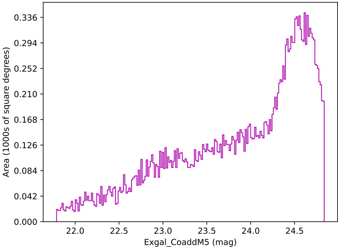
too_elab_r32_d3_giz_v3.4_10yrs Yr 3-4 z band: Exgal_CoaddM5
