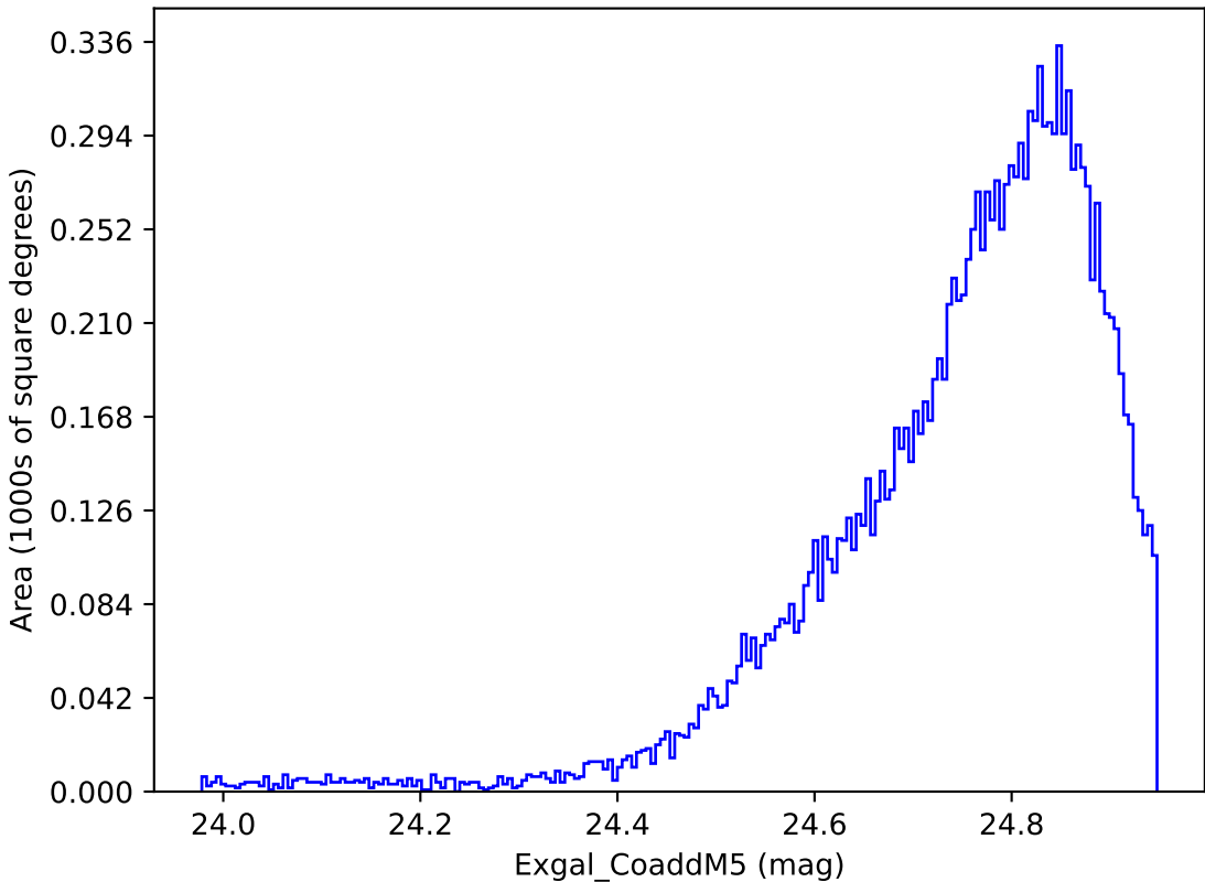
too_elab_r32_d3_giz_v3.4_10yrs WFD y band: Exgal_CoaddM5
