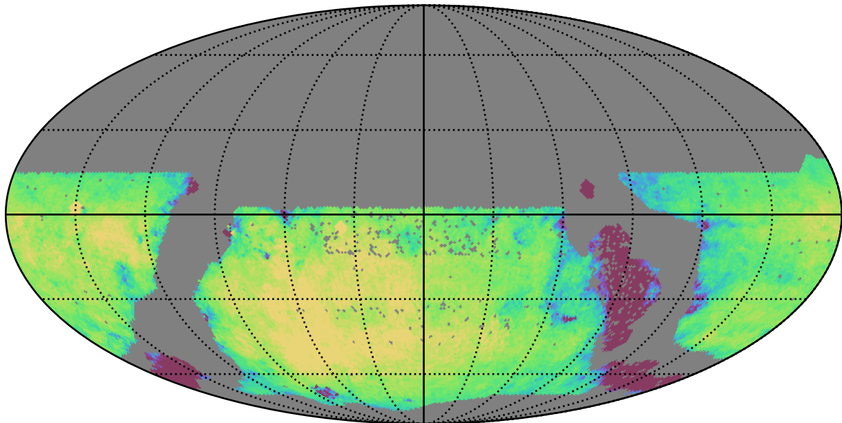
too_elab_r32_d3_giz_v3.4_10yrs WFD g band: Exgal_CoaddM5
