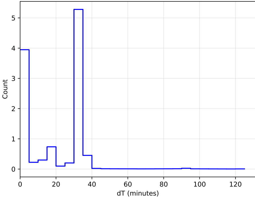
too_elab_r32_d3_giz_v3.4_10yrs WFD: DeltaT Histogram
