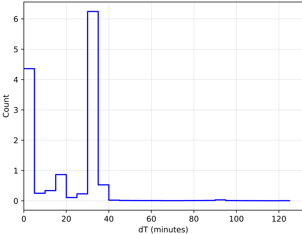
too_elab_r32_d3_giz_v3.4_10yrs All sky: DeltaT Histogram 1e6
