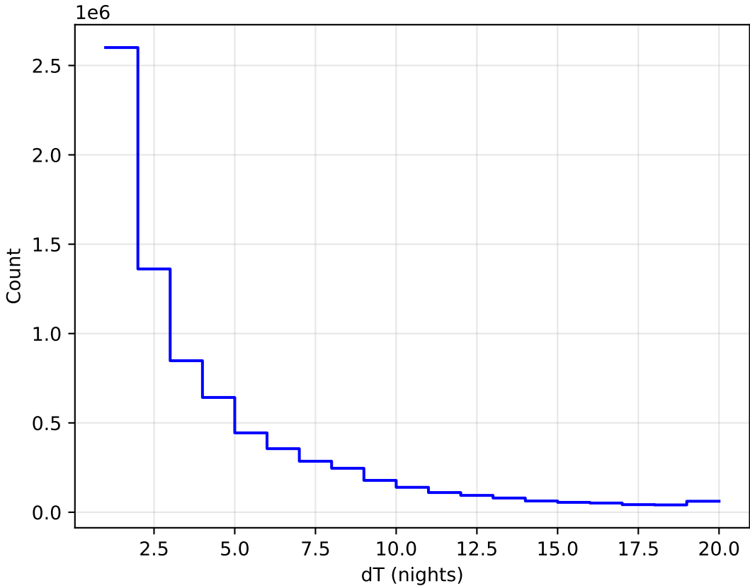
too_elab_r32_d3_giz_v3.4_10yrs WFD all bands: DeltaNight Histogram
