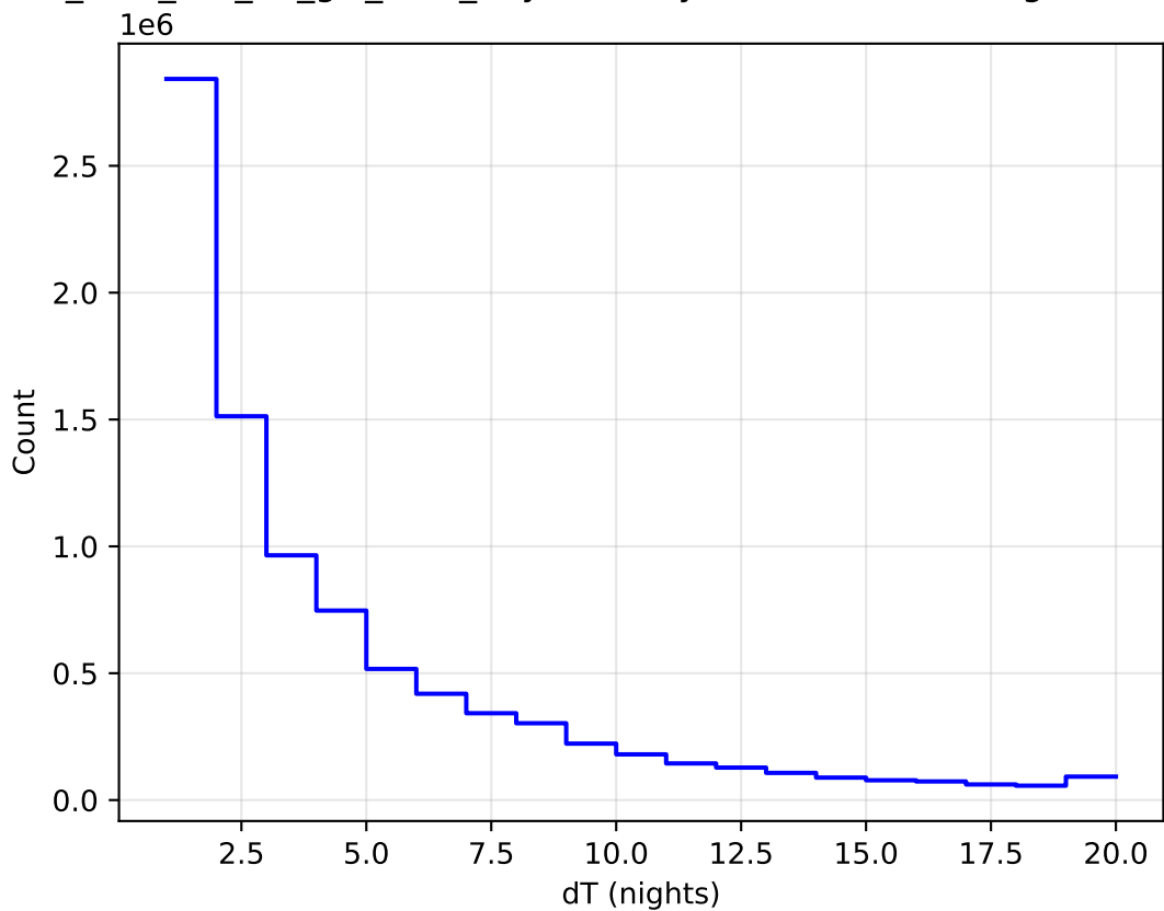
too_elab_r32_d3_giz_v3.4_10yrs All sky all bands: DeltaNight Histogram
