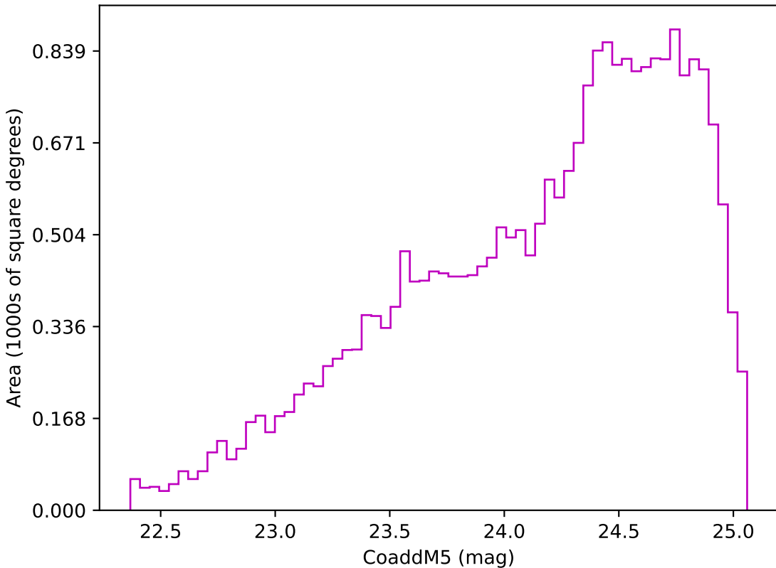
too_elab_r32_d3_giz_v3.4_10yrs Yr 3-4 z band: CoaddM5
