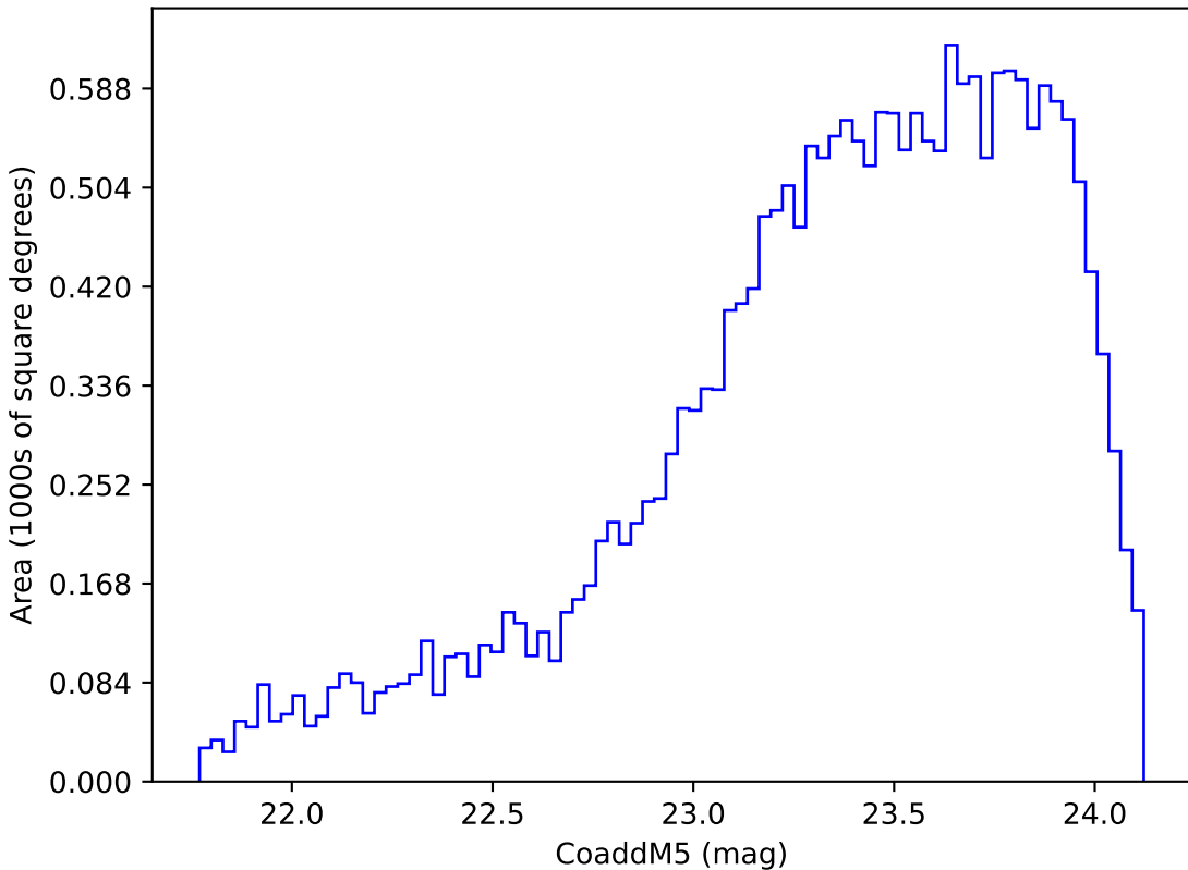
too_elab_r32_d3_giz_v3.4_10yrs Yr 3-4 y band: CoaddM5
