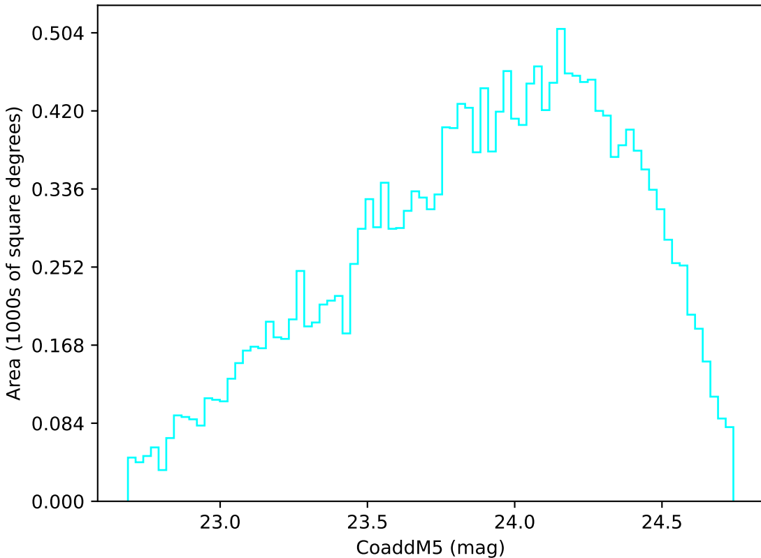
too_elab_r32_d3_giz_v3.4_10yrs Yr 3-4 u band: CoaddM5
