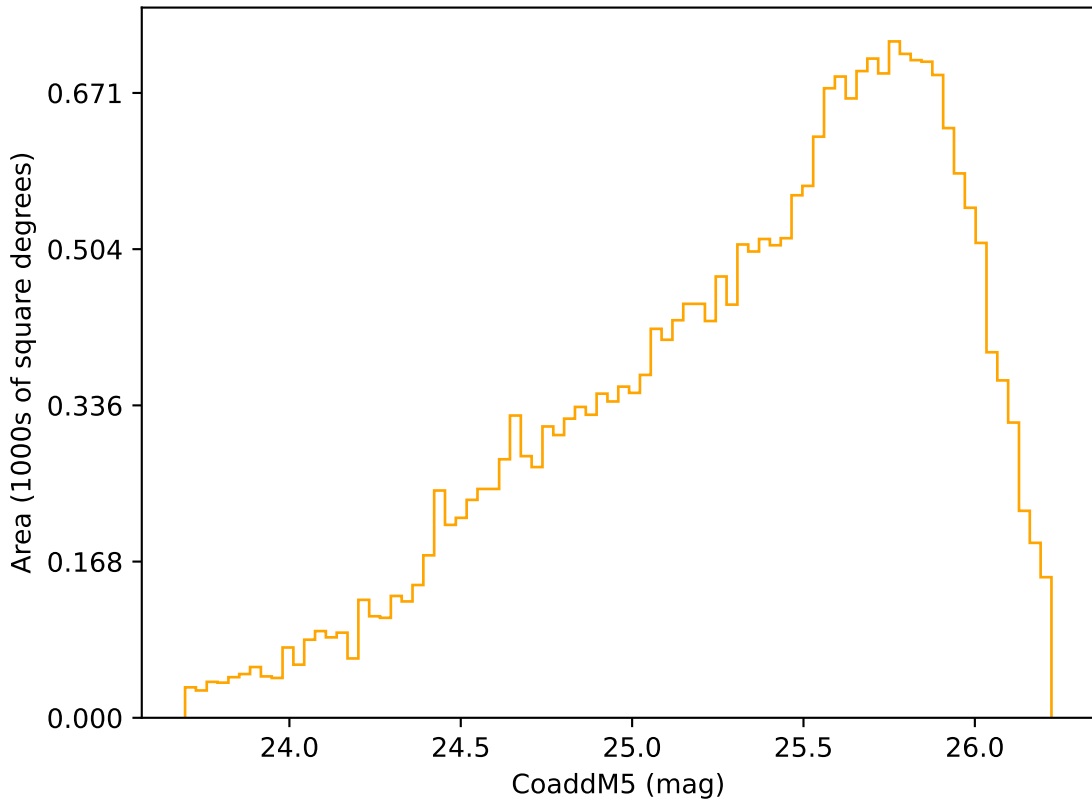
too_elab_r32_d3_giz_v3.4_10yrs Yr 3-4 r band: CoaddM5
