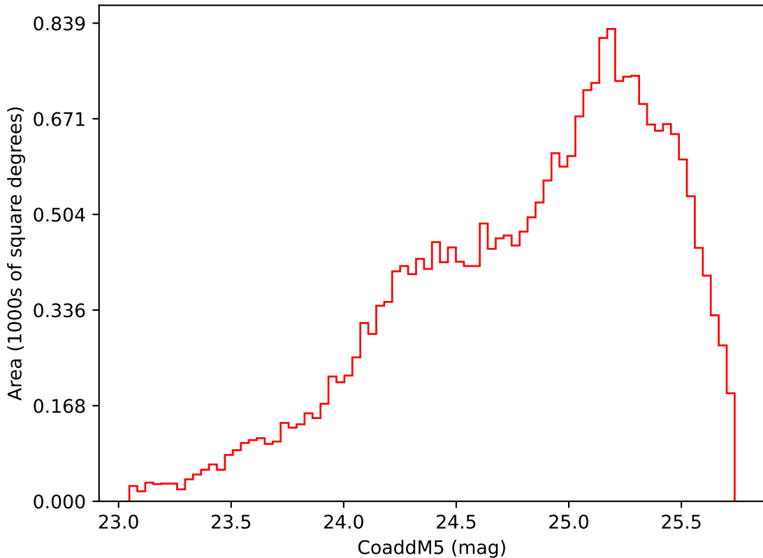
too_elab_r32_d3_giz_v3.4_10yrs Yr 3-4 i band: CoaddM5
