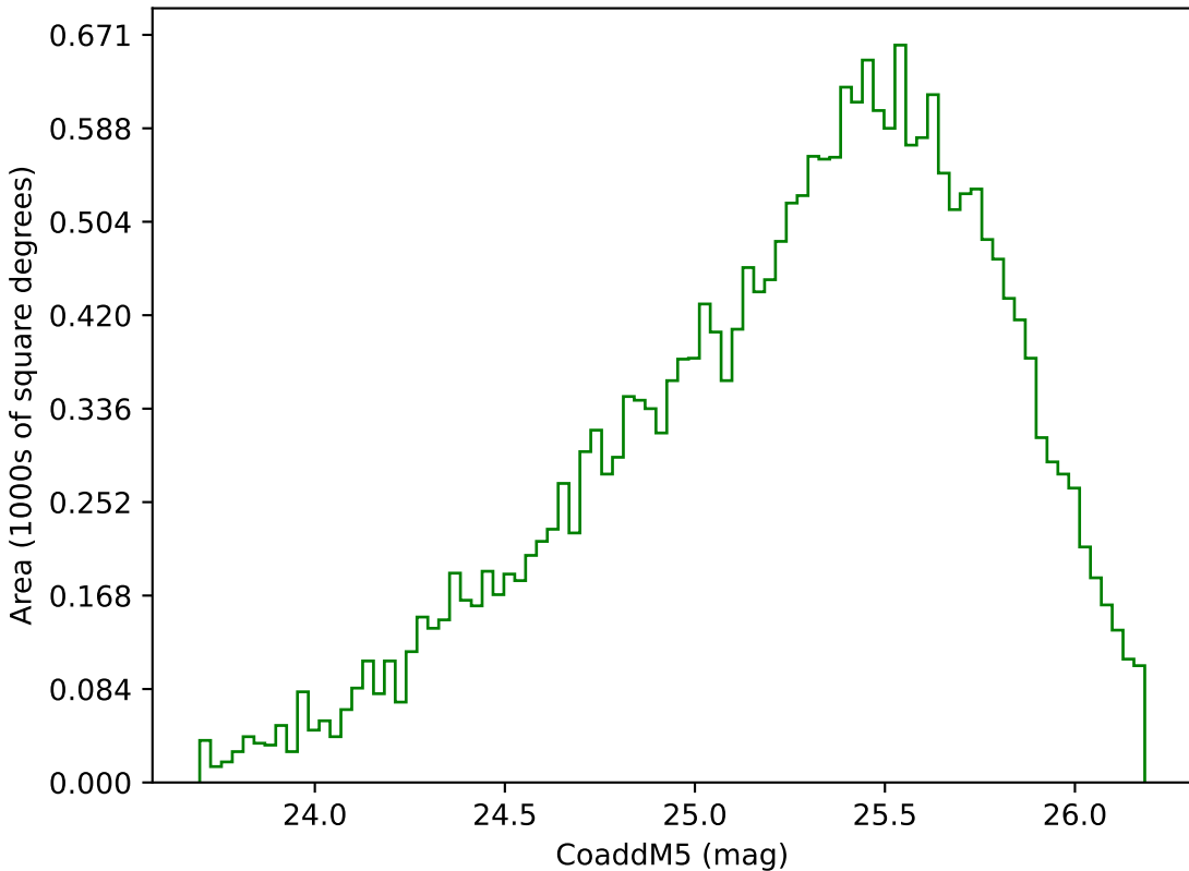
too_elab_r32_d3_giz_v3.4_10yrs Yr 3-4 g band: CoaddM5
