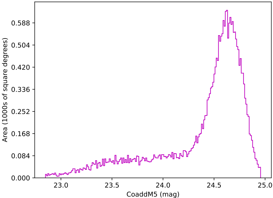
too_elab_r32_d3_giz_v3.4_10yrs Yr 1 z band: CoaddM5
