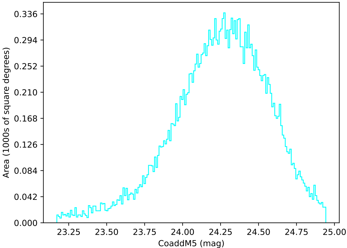
too_elab_r32_d3_giz_v3.4_10yrs Yr 1 u band: CoaddM5
