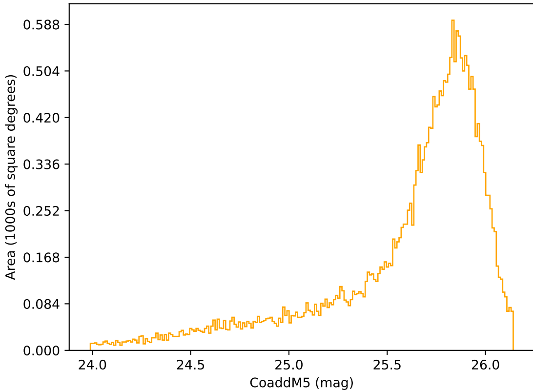
too_elab_r32_d3_giz_v3.4_10yrs Yr 1 r band: CoaddM5
