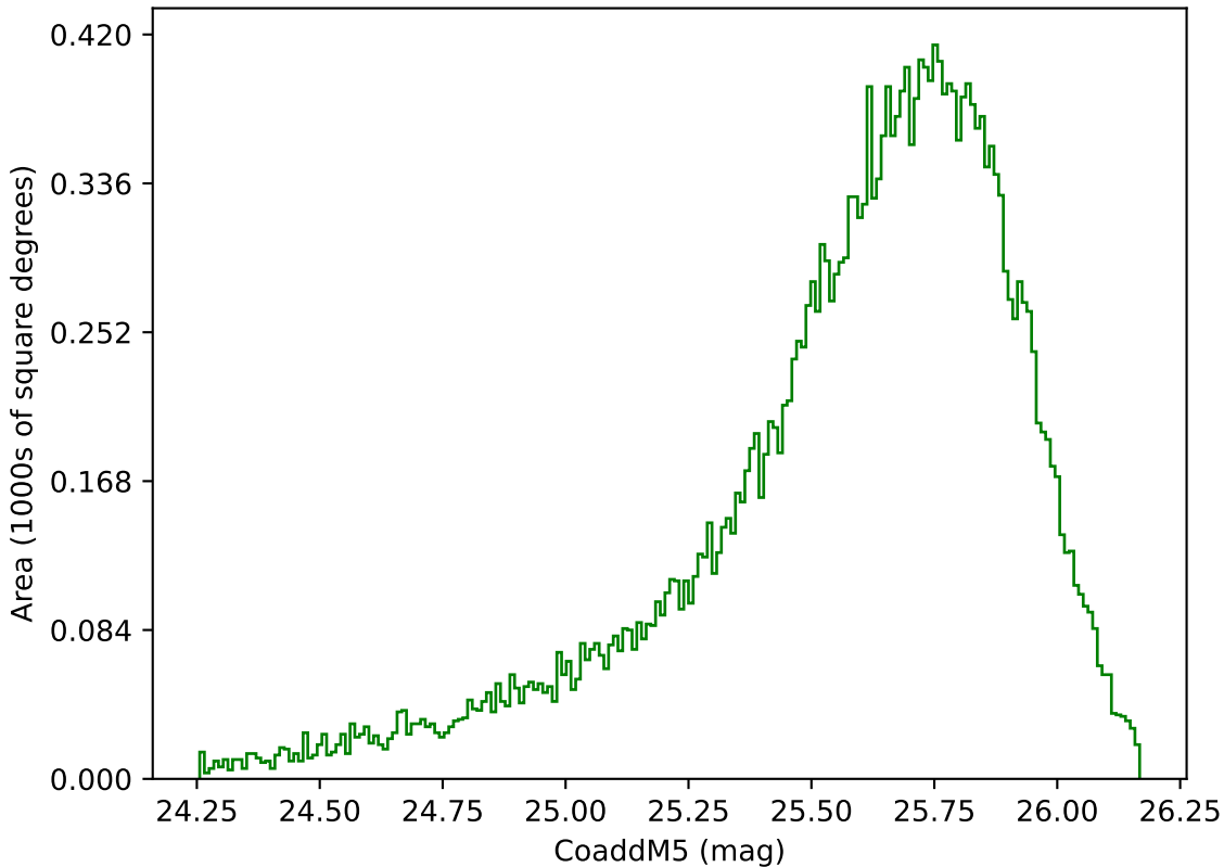
too_elab_r32_d3_giz_v3.4_10yrs Yr 1 g band: CoaddM5
